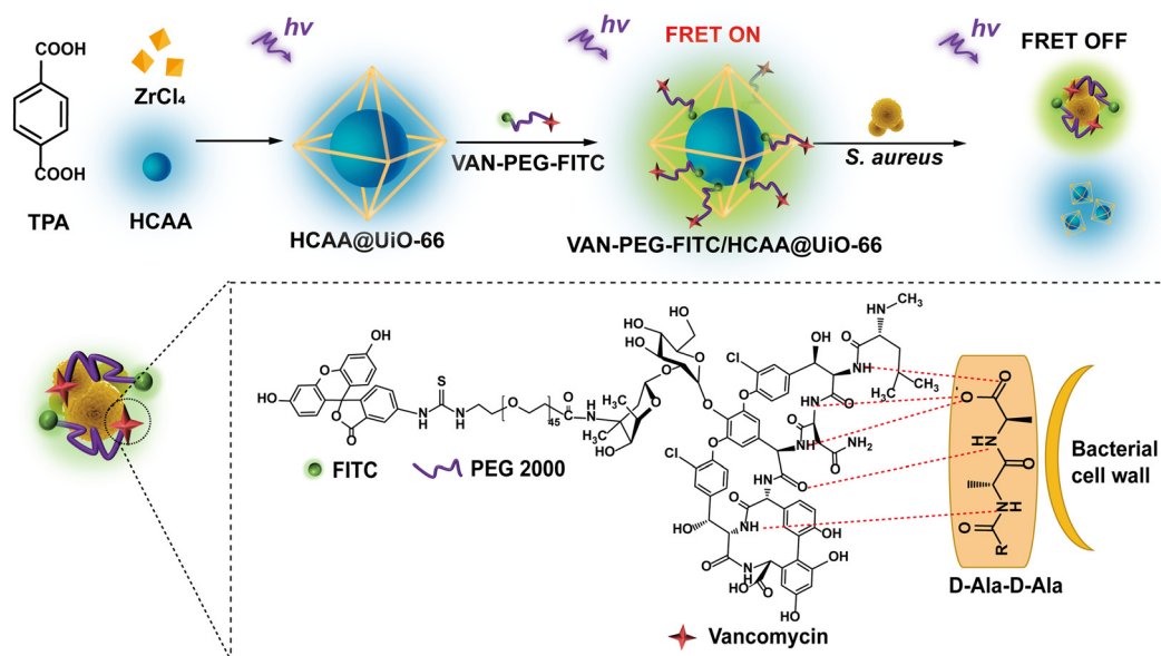
Scheme 1 Schematic interpretation of the FRET ratiometric fluorescent detection of S. aureus using VAN-PEG-FITC/HCAA@UiO-66.
