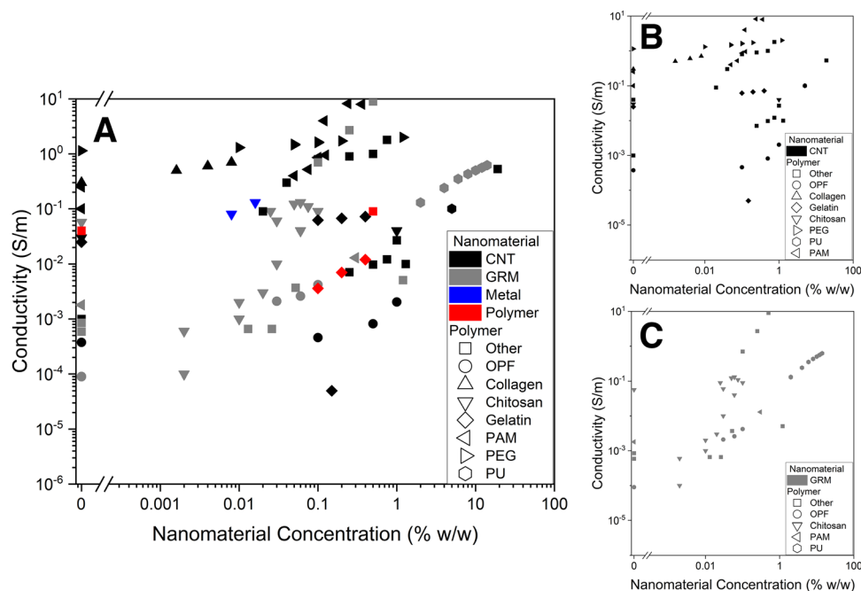
Fig. 15 Nanocomposite hydrogel electrical conductivity vs. nanomaterial concentration. (A) All, (B) CNTs, (C) GRMs. A nanomaterial concentration of 0 represents the electrical conductivity of the pristine hydrogels (without conductive nanomaterials). OPF: oligo(poly(ethylene glycol) fumarate); PAM: polyacrylamide; PEG: polyethylene glycol; PU: polyurethane. Data extracted from ref. 44, 72–74, 87, 88, 91, 109, 111–115, 119, 144, 146, 147, 151, 152, 155–160, 164 and 183.
