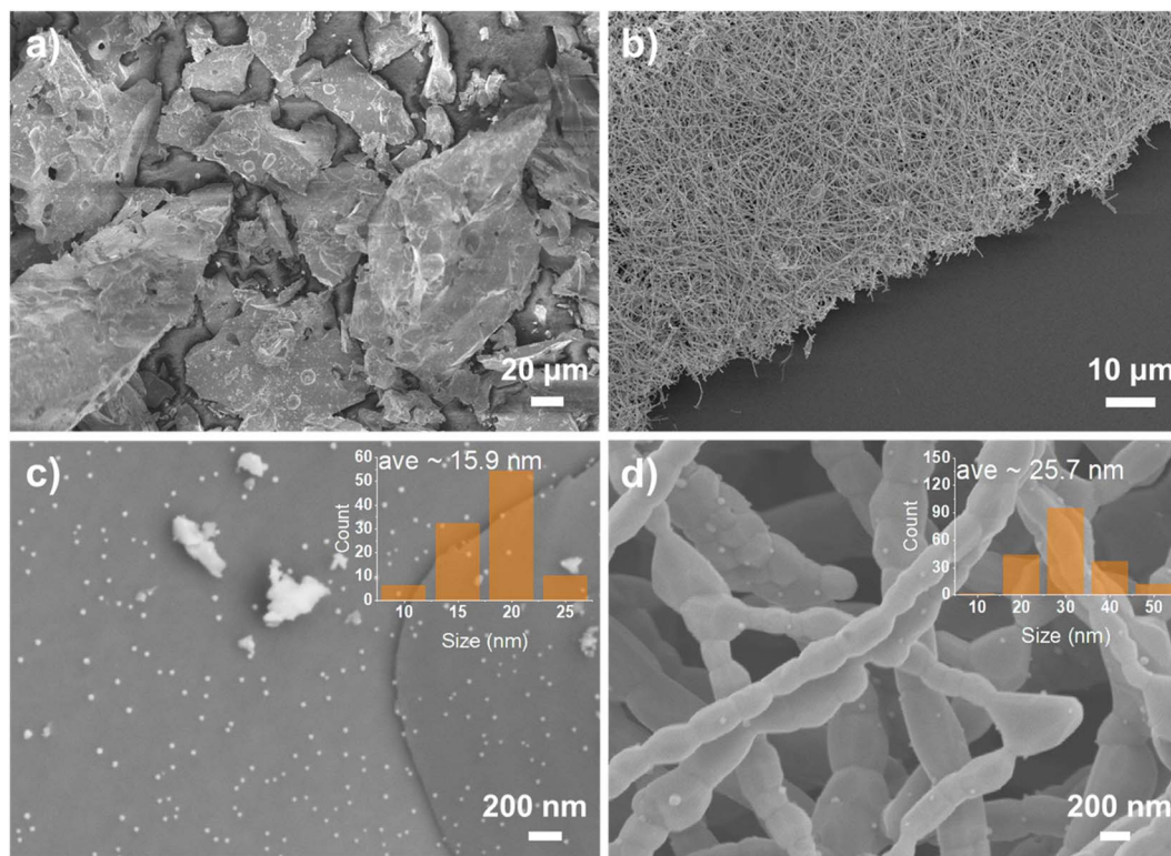
Fig. 2 Morphology of exsolution of Ni nanoparticles from LCNT perovskite materials. SEM figures of (a and c) powder and (b and d) fiber reduced in 5% H_2/N_2 at 800 °C for 4 h. The insets show the size distribution of the exsolved nanoparticles.
