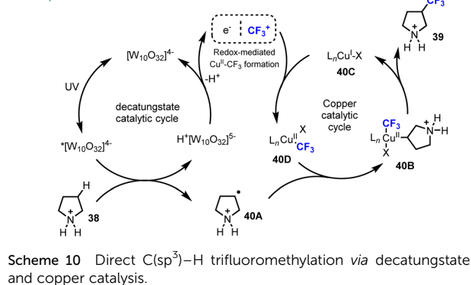
Scheme 11 Decatungstate catalyzed C–H fluoroalkylthiolation.
