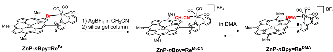
Scheme 2 Synthesis of ZnP-nBpy=ReMeCN and ligand substitution of acetonitrile to DMA.
