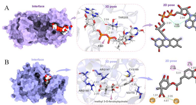
Fig. 12 Binding of potential lead compounds to targets. (A) Docking interface, 3D pose, and 2D pose of the PGK1-FAD complex. (B) Interface, 3D pose, and 2D pose for methyl 3-O-feruloylquininate docking with GSK3 \beta .
