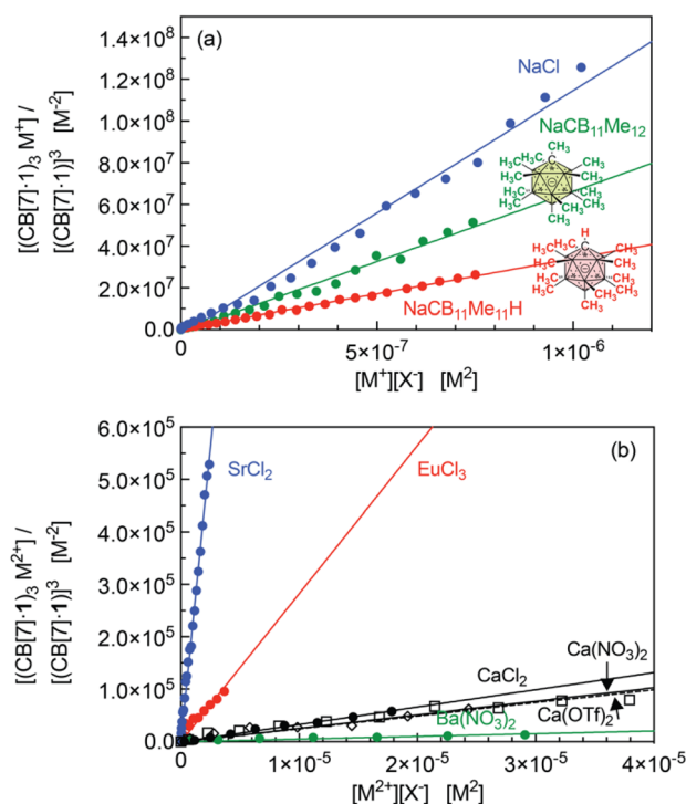
Fig. 7 Plot of [(\text{CB}[7] \cdot 1)_3 \text{M}]/[(\text{CB}[7] \cdot 1)]^3 as a function of [M][X] , for (a) alkali cations M^+ and (b) alkali-earth cations M^{2+} as well as \text{Eu}^{3+} , with linear regressions. Titration affording the best coefficient of determination for each series.
