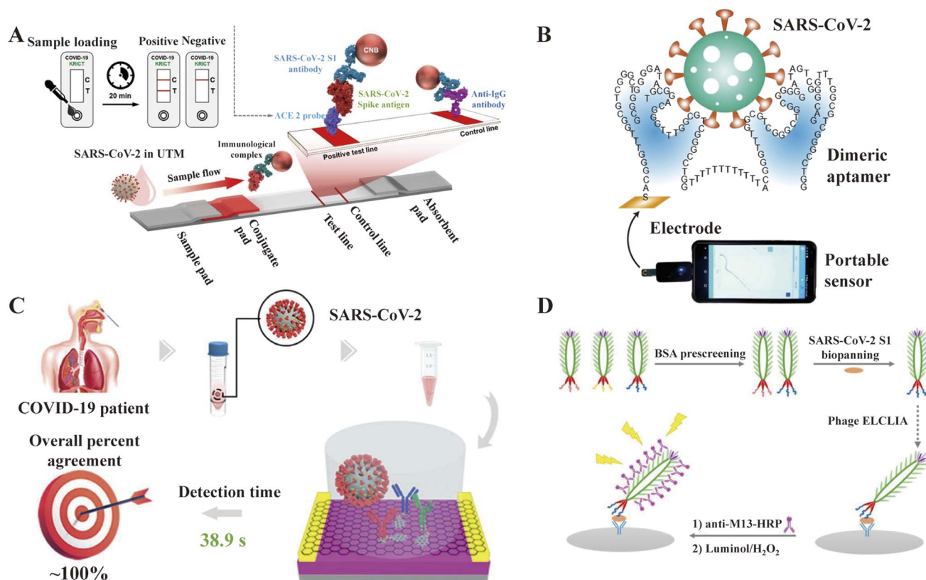
Fig. 14 Schematic diagram of some strategies for S1 protein detection. (A) Schematic of an ACE2-based LFIAs consisting of a sample pad, conjugate pad, nitrocellulose membrane, and absorbent pad. The test line placed on the nitrocellulose membrane contains ACE2 to detect SARS-CoV-2 SP. Reproduced with permission from Biosens. Bioelectron. , 2021, 171 , 112715, 10.1016/j.bios.2020.112715. 374 (B) Platform for the rapid electrochemical detection of S1 protein with high-affinity dimer aptamer. Reproduced with permission from Angew. Chem. , 2021, 60 , 24266–24274, 10.1002/anie.202110819. 388 (C) Multi-antibody FET sensor. Reproduced with permission from J. Am. Chem. Soc. , 2021, 143 , 19794–19801, 10.1021/jacs.1c08598. 386 (D) Schematic diagram of antibody/S1-specific peptide-displayed phage/HRP-M13 antibody-based ELCLIA. Reproduced with permission from Anal. Chem. , 2022, 94 , 11591–11599, 10.1021/acs.analchem.2c01988. 387
