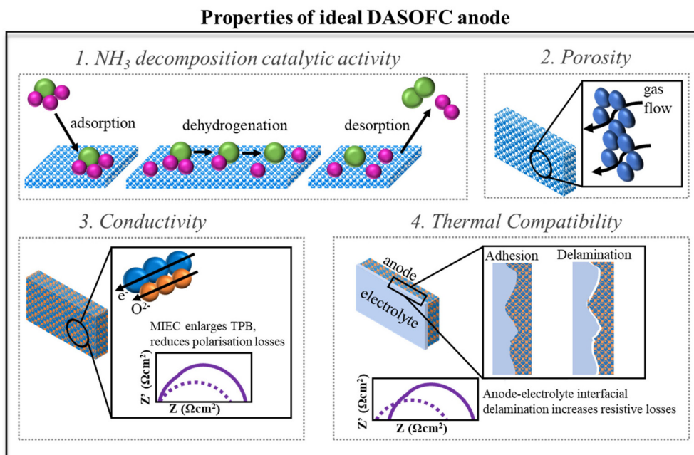
Fig. 7 The schematic shows the four essential properties of the ideal anode material for DASOFC.
