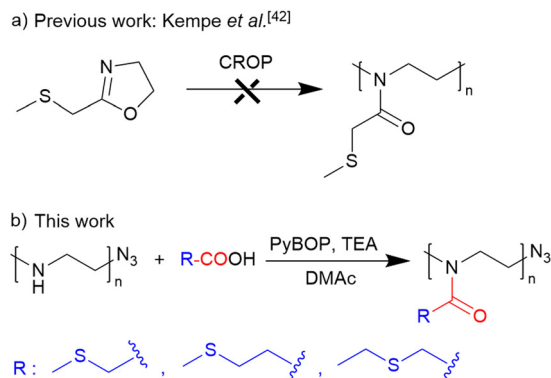
Scheme 1 (a) Schematic representation of the unsuccessful CROP of 2-methylthiomethyl-2-oxazoline 42 and (b) synthesis of thioether-containing homopolymers via acylation of well-defined PEI.
