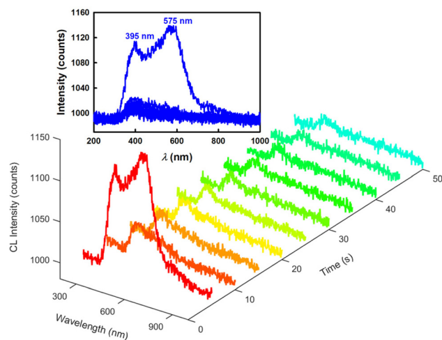
Fig. 3 Spooling CL spectra acquired at a time interval of 5 s in the presence of N-GQD, CPPO and H 2 O 2 . Insets show the 2D view of spooling CL spectra demonstrating constant shapes and peak wavelengths. Reaction conditions: adding 200 \mu L of 1% H 2 O 2 in acetonitrile to 1 mL of an 80% ethyl acetate, 20% acetonitrile solution containing 0.2 mg mL -1 N-GQD, 3.7 mg mL -1 CPPO and 2 mg mL -1 sodium salicylate.
