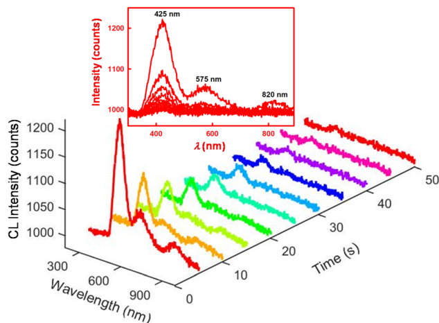
Fig. 2 Spooling CL spectra acquired at a time interval of 5 s in the presence of NS-GQD, CPPO and H 2 O 2 . Inset shows the 2D view of stacked spooling CL spectra demonstrating consistent shapes and peak wavelengths. Reaction conditions: adding 200 \mu L of 1% H 2 O 2 in acetonitrile to 1 mL of an 80% ethyl acetate, 20% acetonitrile solution containing 0.2 mg mL -1 NS-GQDs, 3.7 mg mL -1 CPPO and 2 mg mL -1 sodium salicylate.
