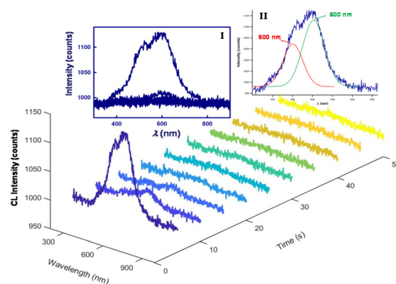
Fig. 4 Spooling CL spectra acquired at a time interval of 5 s in the presence of GQD, CPPO and H 2 O 2 . Insets show the (I) 2D view of spooling CL spectra demonstrating constant shapes and peak wavelengths, and (II) its curve fitting, respectively. Reaction conditions: adding 200 \mu L 1% H 2 O 2 in acetonitrile to 1 mL of an 80% ethyl acetate, 20% acetonitrile solution containing 0.2 mg mL -1 GQD, 3.7 mg mL -1 CPPO and 2 mg mL -1 sodium salicylate.
