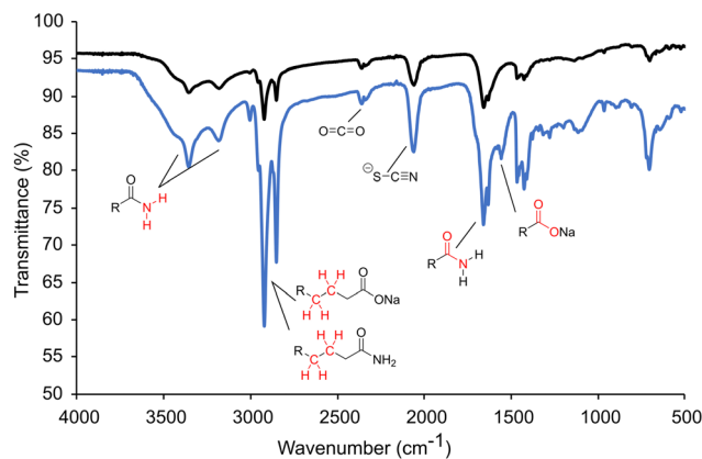
Fig. 4 ATR-FTIR of the nanoparticle solution after centrifugation isolated at low oleate (black) and high oleate (blue).
