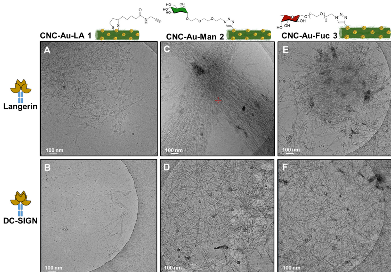
Fig. 3 Cryo-TEM images of the chimera lectins langerin-Fc and DC-SIGN-Fc in TMS treated with a dispersion (0.01% w/w in \text{H}_2\text{O} ) of CNC-Au-LA 1 (A and B), respectively; or CNC-Au-Man 2 (C and D), respectively; or CNC-Au-Fuc 3 (E and F), respectively. Chimera lectins were used at the final concentration of 0.1 \text{ mg mL}^{-1} (ESI†). Buffer TMS: 20 mM TRIS, 150 mM NaCl, 1.0 mM \text{CaCl}_2 , 2.0 mM \text{MgCl}_2 , pH = 8. Scale bar 100 nm.
