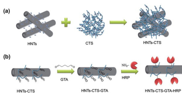
Fig. 19 (a) Stepwise preparation and (b) immobilization of HRP on a chitosan (CTS) matrix. Reproduced from ref. 195 with permission from Elsevier, copyright 2013.
