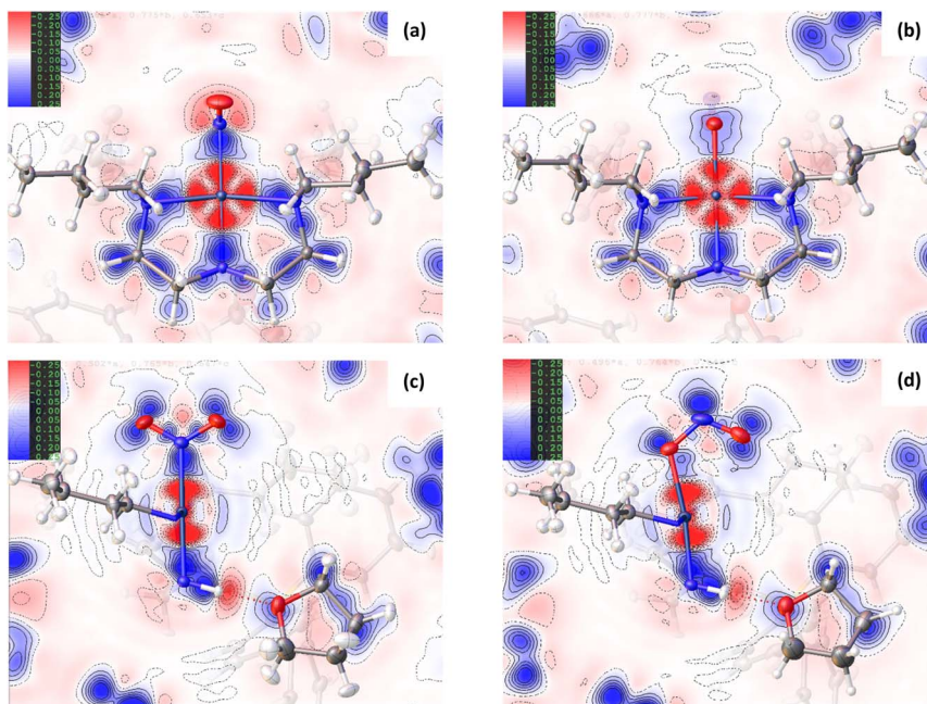
Fig. 1 2D deformation density maps for the ground state (GS) and excited state (ES) structures of complex 1 , showing the residual electron density between the non-spherical atom refinement (HAR) and a standard spherical atom model (IAM) from NoSpherA2. Blue = positive deformation density (e.g. in bonds or lone pairs), red = negative deformation density. (a) GS map in the Pd(1), N(1), N(2), N(3), N(4) square plane, (b) ES map in the Pd(1), N(2), N(3), N(4) square plane, (c) GS map in the Pd(1), N(1), O(1), O(2) plane (plane of the nitro ligand), (d) ES map in the Pd(1), N(1A), O(1A), O(2A) plane (plane of the nitrito ligand).
