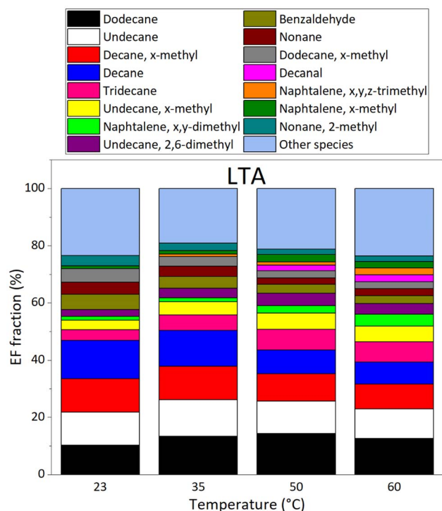
Fig. 7 Evolution of VOC emission composition in % for the species accounting for more than 75% of VOC emissions (EF > 3.63 μg m -2 h -1 for LTA asphalt mixtures) as a function of temperature, as measured by GC-MS/FID under dry (RH = 0.1%) and dark conditions, for the LTA2 old asphalt sample.
