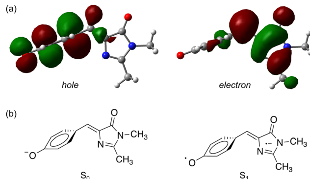
Fig. 5 Natural transition orbitals 83 for the S_1 \leftarrow S_0 transition in p HBDI − : (a) the P-trap minimum energy geometry, (b) schematic illustrations of the resulting ground and excited-state electronic configurations.
