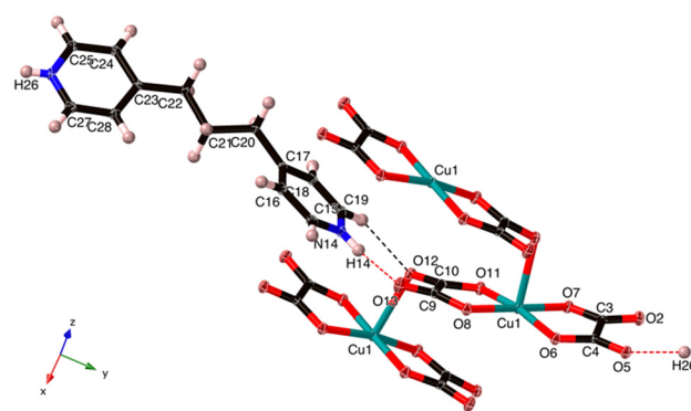
Fig. 4 The asymmetric unit of \text{C}_{13}\text{H}_{16}\text{N}_2[\text{Cu}(\text{C}_2\text{O}_4)_2] ( 2 ) with one extra oxalate, one extra Cu and one additional N–H. The Cu–O7 is 2.538 Å, which is normal for an axial Jahn–Teller bond.
