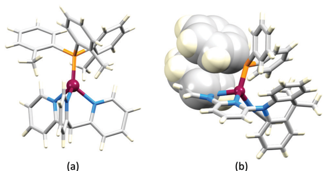
Fig. 21 (a) Structure of the cation in [\text{Cu}\{\text{P}(2\text{-MeC}_6\text{H}_4)_3\}(\text{27})][\text{PF}_6] (CSD refcode HIRJEA). (b) The structure of [\text{Cu}(\text{PPh}_3)(\text{28})(\text{NCMe})]^+ in the [\text{BF}_4]^- salt (refcode NAVFUO) showing \pi -stacking between one phenyl ring of \text{PPh}_3 and the phenyl ring of 28 .
