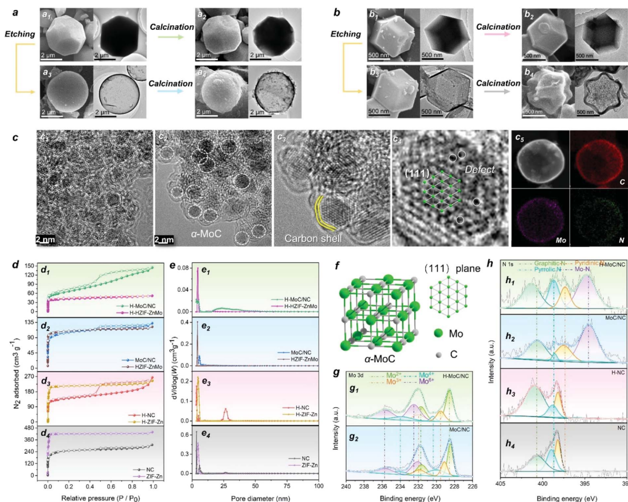
Fig. 2 (a) SEM and TEM images of HZIF-ZnMo ( a_1 ), MoC/NC ( a_2 ), H-HZIF-ZnMo ( a_3 ) and H-MoC/NC ( a_4 ). (b) SEM and TEM images of ZIF-Zn ( b_1 ), NC ( b_2 ), H-ZIF-Zn ( b_3 ) and H-NC ( b_4 ). (c) Hetero-interfaces in HR-TEM ( c_1 ), the MoC nanoparticles ( c_2 ), MoC@C structure ( c_3 ), lattice and defects ( c_4 ) and EDS mapping ( c_5 ) images of H-MoC/NC. (d) N_2 -sorption isotherms curves. (e) Pore diameter distribution curves. (f) Crystalline structure of \alpha -MoC. (g) Mo 3d XPS spectra for H-MoC/NC and MoC/NC. (h) N 1s XPS spectra for H-MoC/NC, MoC/NC, H-NC and NC.
