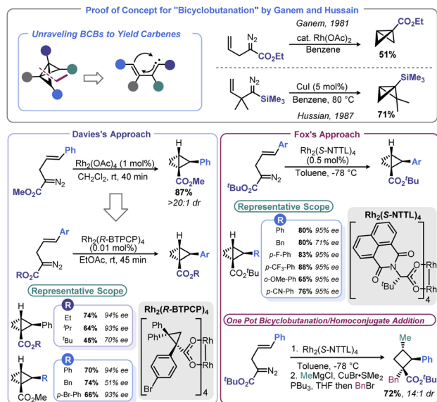
Scheme 3 BCB synthesis via metal-mediated intramolecular [2 + 1] bicyclobutination.
