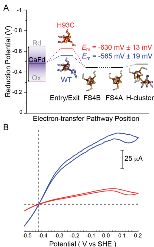
Fig. 3 (A) Thermodynamic landscape for electron transfer between the catalytic H-cluster in CaI and its redox partner ferredoxin. The scheme shows E_m values for the distal [\text{4Fe-4S}] cluster of WT CaI (blue) and H93C CaI (red) obtained in this study, in relation to the E_m range for reduced (Rd) and oxidized (Ox) CaFd, 21 the E_m 's of F-cluster relay comprised of [\text{4Fe-4S}] clusters FS4B and FS4A, and the formal potential of the H-cluster at pH 8.8. 19 (B) Electrocatalytic profiles of CaI WT (blue) and CaI H93C (red). Voltammograms were collected under 1 atm of \text{H}_2 at a potential scan rate of 1 \text{ mV s}^{-1} . Other experimental conditions are pH 7.0, 25^\circ\text{C} and an electrode rotation rate of 3500 rpm. The dotted horizontal line shows zero current.
