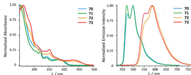
Fig. 14 (Left): normalised UV-vis absorption spectra of 70–73 in THF; (right): normalised emission spectra of 70–73 recorded in a PS film (5 wt%) at 298 K ( \lambda_{\text{ext}} 385 for 70 and 71 and 420 nm for 72 and 73 ). Adapted with permission from ref. 118. Copyright (2021) The Royal Society of Chemistry.
