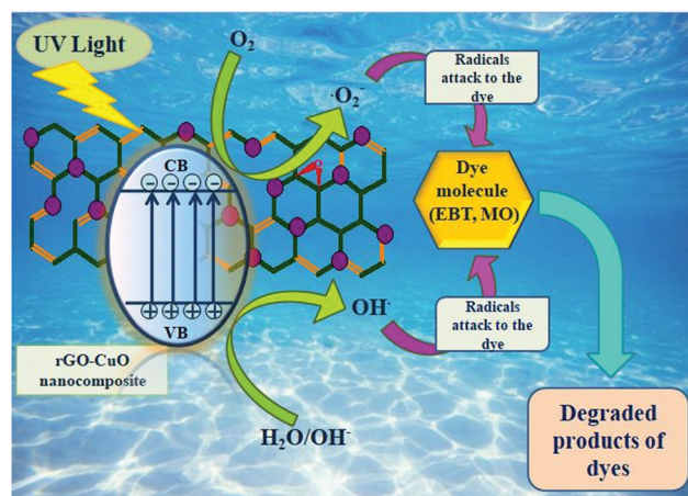
Fig. 11 A plausible mechanism for organic pollutant removal over the CuO/rGO nanocomposite.
