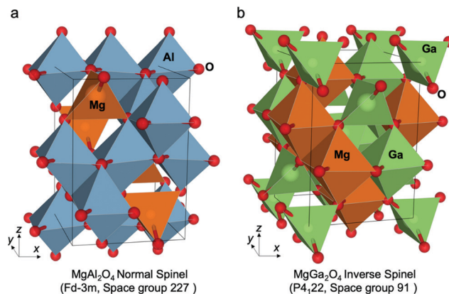
Fig. 36 Normal and inverse spinel structures. (a) MgAl_2O_4 normal and (b) MgGa_2O_4 inverse ground state atomic configurations. In each case the unit cell is shown by solid black lines. Octahedral and tetrahedral atomic coordination environments are also identified by the coordination polyhedra in each case. Reproduced with permission from ref. 717. Copyright Nature Publishing 2020.
