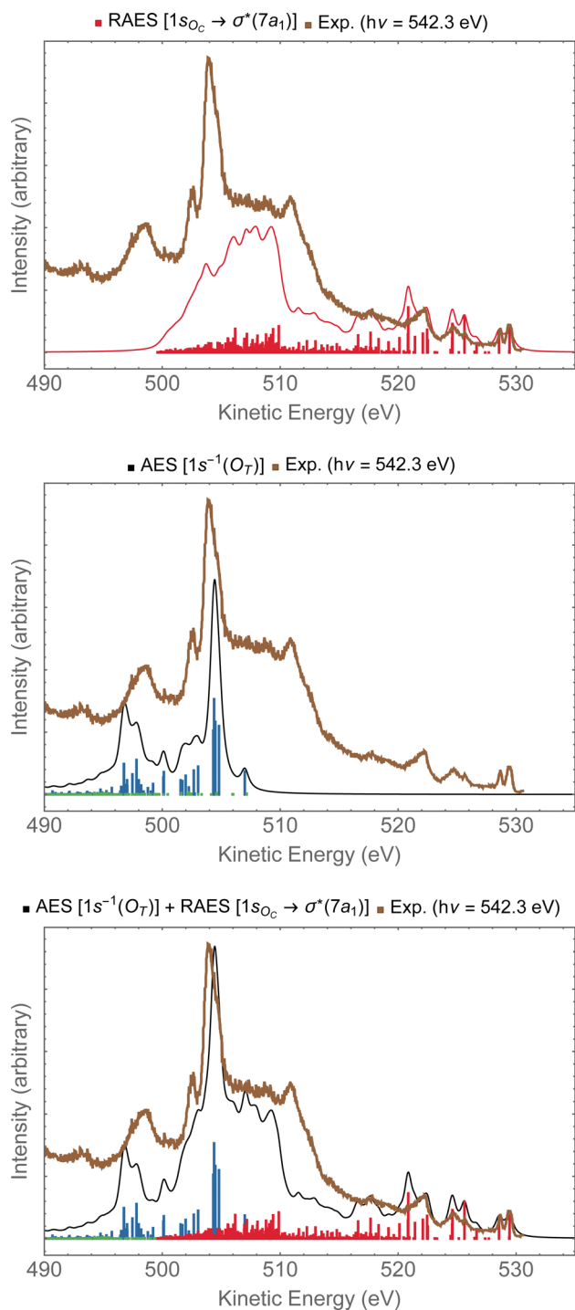
Fig. 9 In the top panel, the RAES of \text{O}_3 at the 1s_{\text{O}_c} \rightarrow \sigma^*(7a_1) resonance is plotted alongside with the experimental spectrum. 13 In the middle panel, the AES at the 1s_{\text{O}_r}^{-1} edge is shown. In the bottom panel, the sum of AES and RAES contributions are plotted. The computed spectra (RAES and AES) were shifted by +1.3 eV and broadened with Lorentzian functions with \text{fwhm} = 0.30 eV. The experimental data were digitized from ref. 13.
