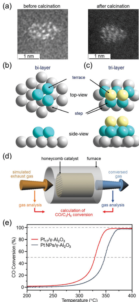
Fig. 18 (a) HAADF-STEM images of \text{Pt}_{17}(\text{PPh}_3)_8(\text{CO})_{12}/\gamma\text{-Al}_2\text{O}_3 (left) and \text{Pt}_{17}/\gamma\text{-Al}_2\text{O}_3 (right). Two proposed structures for \text{Pt}_{17} on \gamma\text{-Al}_2\text{O}_3 based on the HAADF-STEM images of \text{Pt}_{17}/\gamma\text{-Al}_2\text{O}_3 : (b) bi-layer and (c) tri-layer. In (b) and (c), both top and side views are shown. (d) Schematic illustration of estimation of CO and \text{C}_3\text{H}_6 conversion over \text{Pt}_{17}/\gamma\text{-Al}_2\text{O}_3 or Pt NPs/ \gamma\text{-Al}_2\text{O}_3 coated on a cordierite honeycomb substrate. (e) CO conversion over \text{Pt}_{17}/\gamma\text{-Al}_2\text{O}_3 (red curve) and Pt NPs/ \gamma\text{-Al}_2\text{O}_3 (gray curve). Reproduced from ref. 299. Copyright 2020 The Royal Society of Chemistry.
