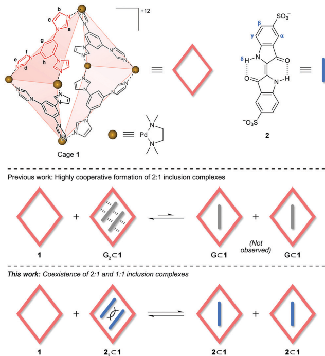
Fig. 1 Structural formulae of cage 1 and indigo carmine 2 (top) and schematic illustration of equilibria between 2:1 and 1:1 inclusion complexes (bottom). Counterions = NO 3 - for 1 and Na + for 2 .
