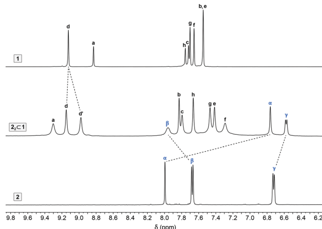
Fig. 2 Partial 1 H NMR spectra of cage 1 (top), indigo carmine 2 (bottom), and 2 < 1 (middle) (500 MHz, D 2 O, 298 K). For the full-range spectrum of 2 < 1 , see Fig. S2 in the ESI†.
