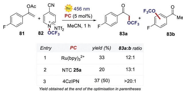
Scheme 37 Radical α-trifluoromethoxylation of ketones.
