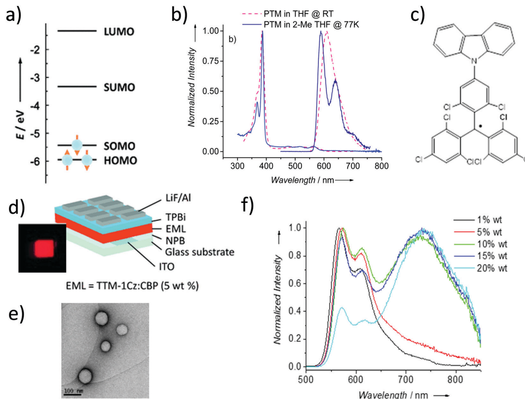
Fig. 6 (a) Schematic representation of the frontier orbitals of PTM radicals. (b) Absorption and emission of PTM in THF at room temperature ( \phi_F = 0.02 ) and 2-methyl THF at 77 K ( \phi_F = 0.72 ). (c) Molecular structure of the TTM-1Cz. (d) Device architecture of the OLED based on TTM-1Cz. The inset shows a picture of the TTM-1Cz-based OLED operating at 7 V. Reprinted with permission from ref. 92. Copyright 2015 Wiley-VCH. (e) TEM image of PTMd-ONPs. (f) Normalized emission spectra of TTMd-ONPs. Reprint with permission from ref. 108. Copyright 2017 Royal Society of Chemistry.
