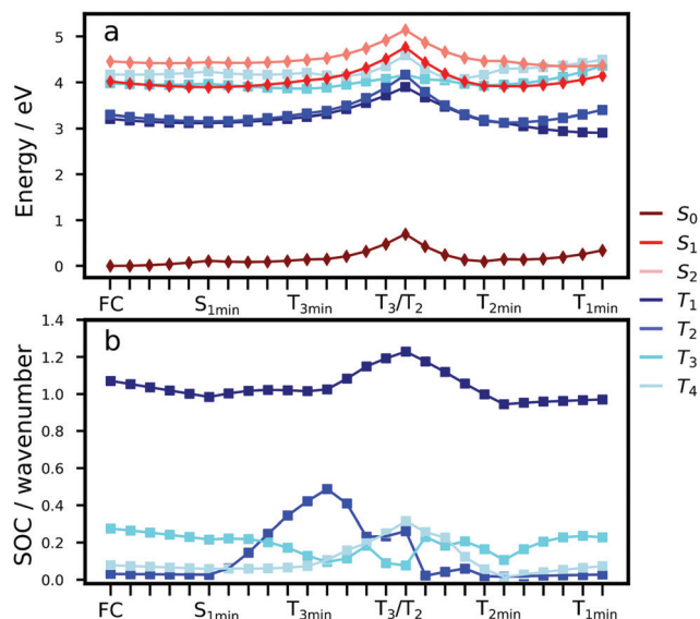
Fig. 2 (a) Linear interpolated Cartesian coordinate (LIICC) pathway from the Franck–Condon (FC) geometry, to S_1 , to the excited state minima (OEC model, TD-B3LYP/6-311++G(d,p)). (b) Spin–orbit coupling values along the LIICC pathway.
