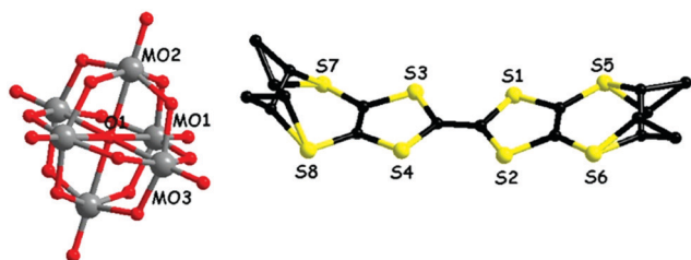
Fig. 4 Detail of the crystal structure of [(\text{rac})\text{-}1]_2(\text{Mo}_6\text{O}_{19}) . Both ethylene bridges of the donor are disordered. Hydrogen atoms have been omitted.
