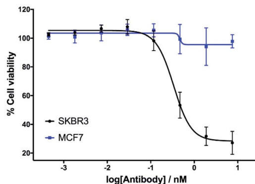
Fig. 6 The in vitro evaluation of ADC mAb 1 -8-14 in HER2-positive cells (SKBR3) and HER2-negative cells (MCF7). Viability data shows the mean of three independent experiments and error bars represent standard error of the mean.
