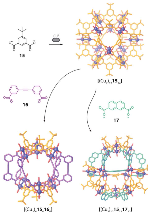
Fig. 8 Ligand substitution transforms homoleptic rhombic cuboctahedron [(Cu_2)_{12}15_{24}] into heteroleptic cages [(Cu_2)_615_616_6] and [(Cu_2)_{12}15_{12}17_{12}] when using bent dicarboxylate ligands.
