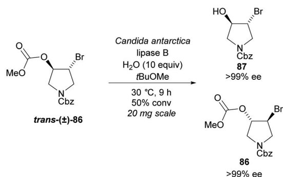
Scheme 22 Hydrolysis of various disubstituted pyrrolidines.
