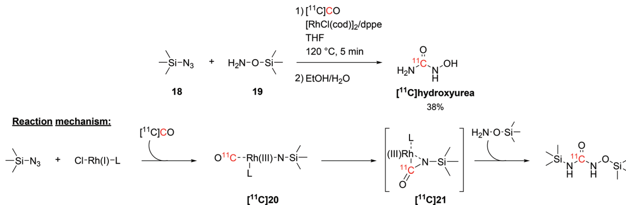
Scheme 10 Coupling of ^{11}\text{C} CO with trimethylsilyl precursors to yield ^{11}\text{C} hydroxyurea. 58
