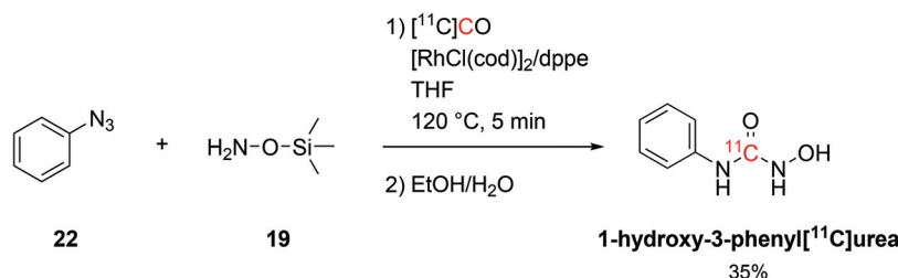
Scheme 11 Synthesis of 1-hydroxy-3-phenyl ^{11}\text{C} urea. 58
