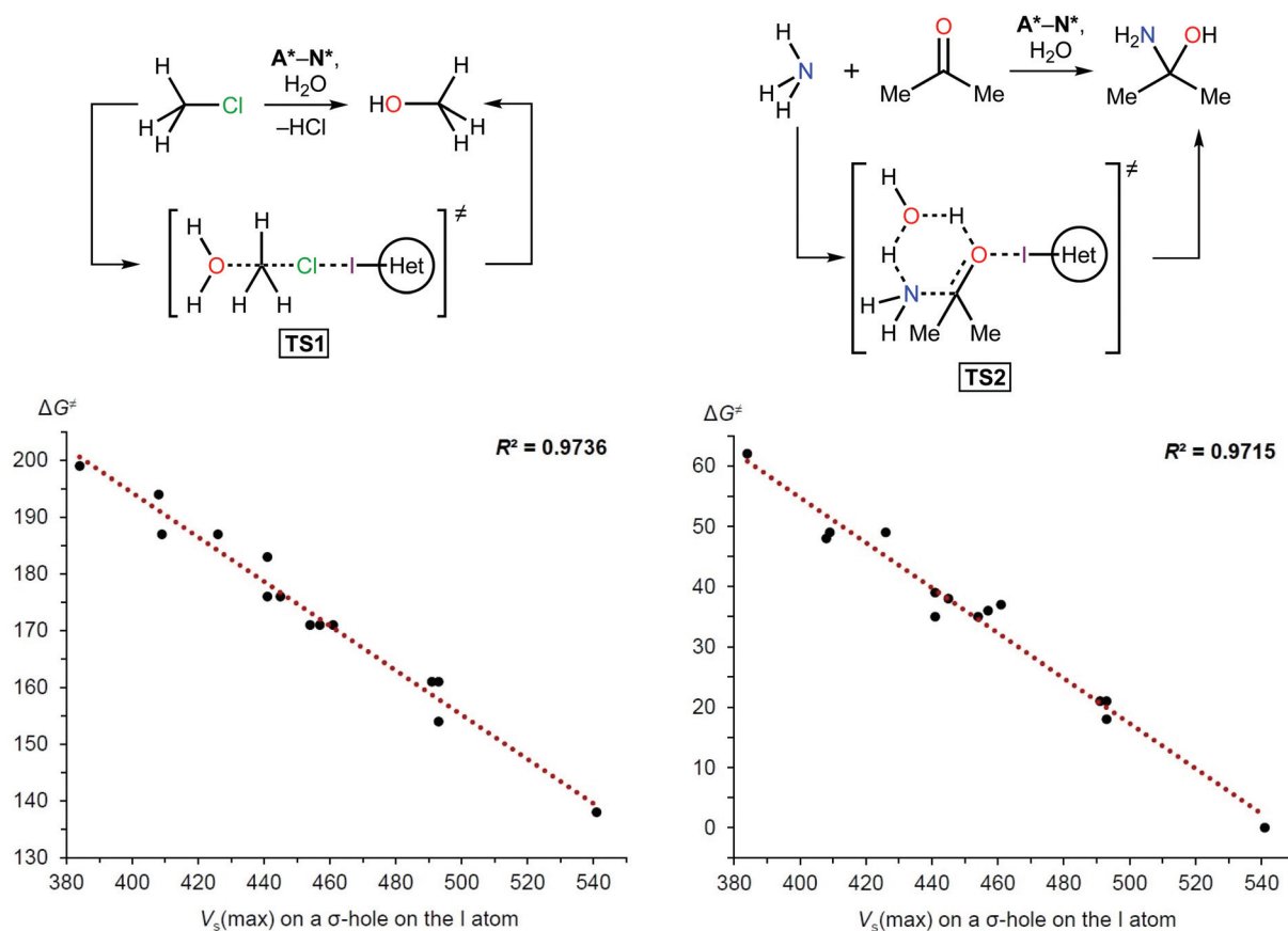
Scheme 1 Model reactions (top) and plots showing the correlation between the Gibbs free energy of activation ( \Delta G^\ddagger ; kJ mol -1 ) and V_s(\text{max}) on the I atom \sigma -hole (kJ mol -1 ).
