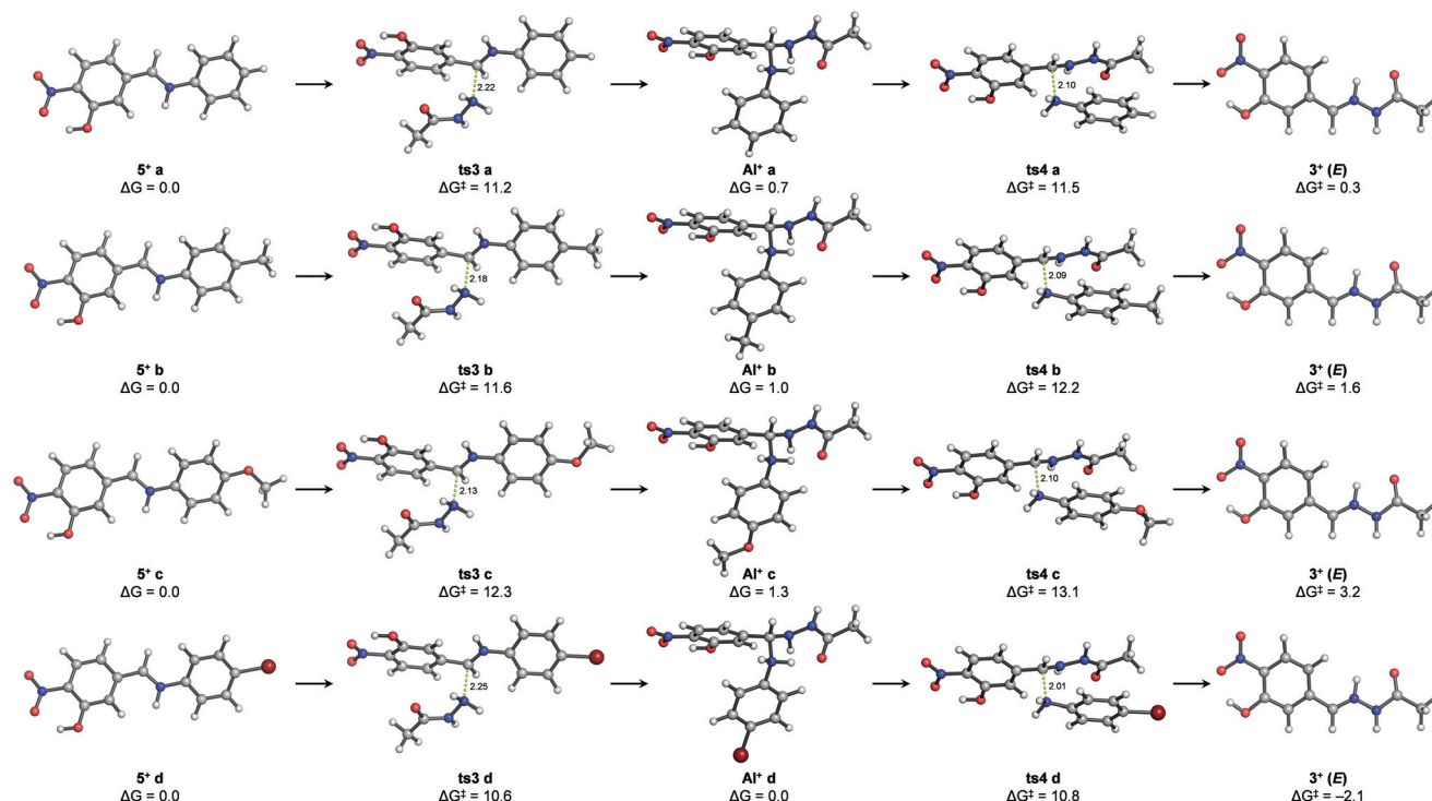
Fig. 5 Lowest-energy structures calculated with SMD(CH 3 CN)/M06-2X/6-311++G(2d,p)//PCM(CH 3 CN)/M06-2X/6-31+G(d,p) for the nucleophilic addition of acylhydrazide to iminium derivatives 5 + a–d (ts3 a–d ), the corresponding protonated aminal intermediates ( Al + a–d ) and subsequent water elimination (ts4 a–d ) to yield hydrazone 3 + (E) (only the E isomer is shown). Relative free energies ( \Delta G ) from the separated reactants are given in kcal·mol −1 and distances are given in Angstrom.
