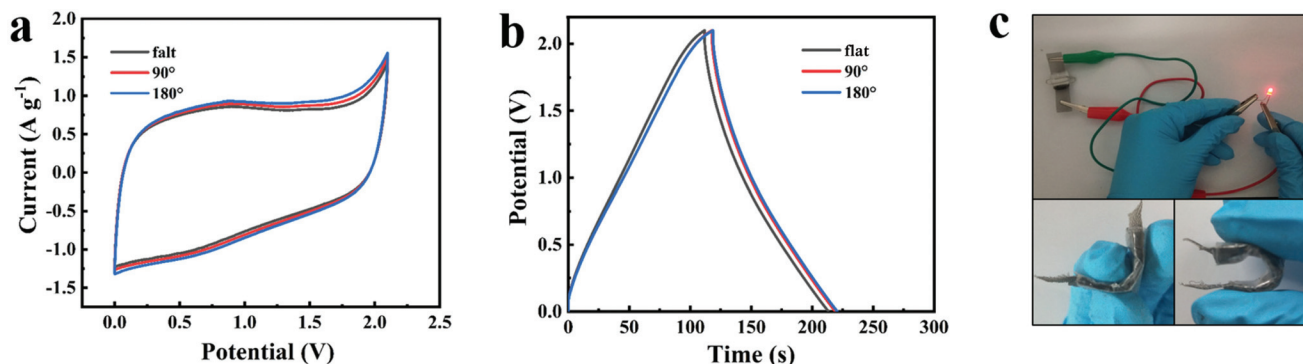
Fig. 6 CV curves at 10 \text{ mV s}^{-1} (a) and GCD profiles at 1 \text{ A g}^{-1} (b) of the assembled flexible device at 0\text{--}180^\circ . Optical images of the flexible device under different bending conditions (c).
