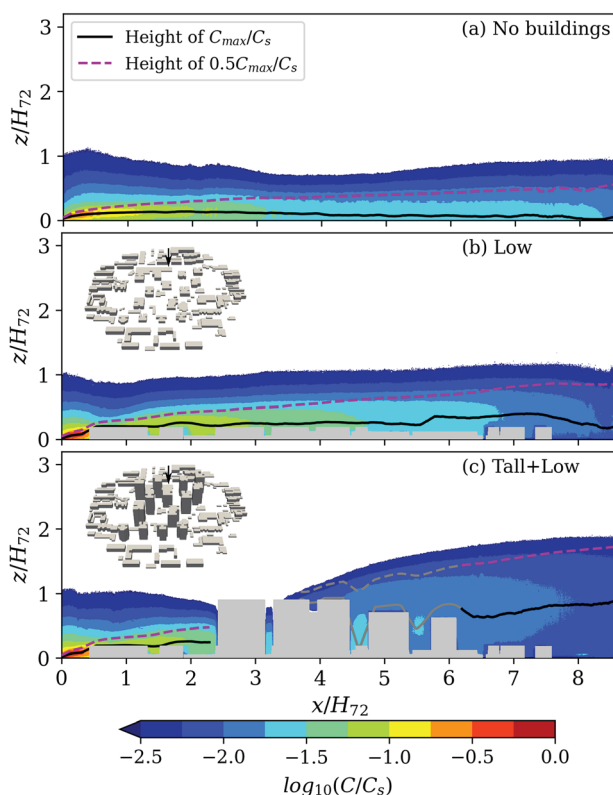
Fig. 6 Contours of scaled tracer concentrations ( \log_{10}(C/C_s) ) in the (x, z) plane in the surface layer for areas (a) without buildings, (b) with a Low configuration without the tall-building cluster, and (c) Tall + Low ( i.e. tall building cluster with the surrounding low-rise buildings in the Beijing neighbourhood). For (b and c) the forcing wind direction is from the north ( \theta = 0^\circ ; arrows in insets of building geometries). The heights of the maximum concentration ( C_{\max}/C_s ; solid lines) and of 0.5C_{\max}/C_s (dashed lines) are indicated. In (c) grey lines indicate when values are less reliable, as tall buildings block the camera view. All spatial dimensions are scaled by the height of the tallest building in the cluster ( H_{72} = 72 m). The tracer source is located at x/H_{72} = 0 .
