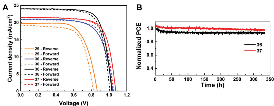
Fig. 11 (A) Reverse J - V curves of the champion PSCs of composition No. 29, 30, 36, and 37 using 1.0 M perovskite precursor solutions with 5% excess Pb ^{2+} . (B) Continuous MPP tracking results under 1 Sun irradiation in a N _2 atmosphere for devices of composition No. 36 and 37.
