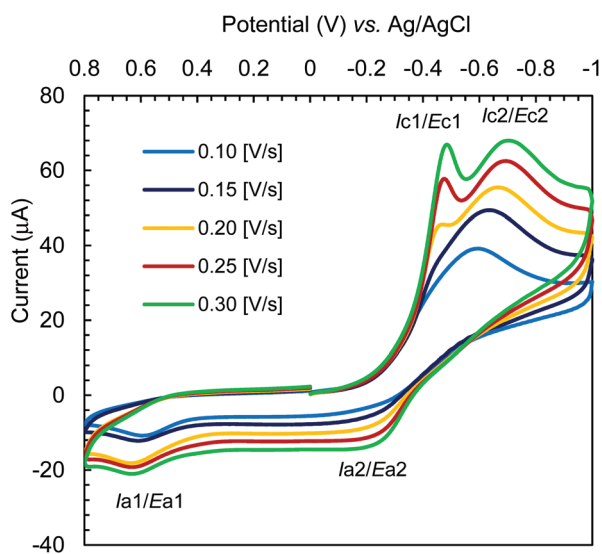
Fig. 10 Cyclic voltammograms for \text{Cu-R-L}^1 ( 0.5 mM); TBAP ( 0.1 M) at varying scan rates 0.10\text{--}0.30 V \text{s}^{-1} in acetonitrile at 25 °C.
