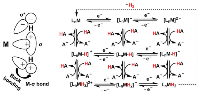
Scheme 25 Schematic presentation of the formation of M-H_2 \sigma bond and M_{d\pi} \rightarrow H_2 backdonation (left). Possible mechanistic pathways for catalytic reduction of proton to hydrogen in the natural hydrogenases or synthetic catalysts (right).
