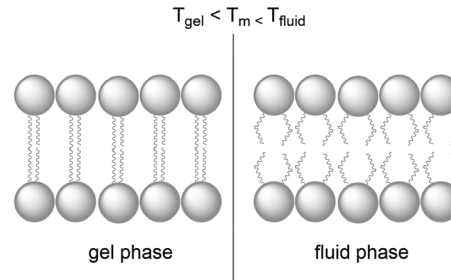
Fig. 8 A lipid bilayer changes from the rigid gel phase (left) to the mobile fluid phase (right) above the transition temperature ( T_m ) of the lipid.
