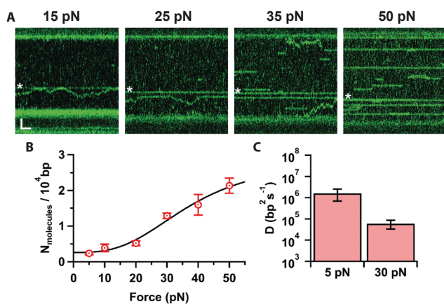
Fig. 4 (A) Kymographs of force stretched \lambda -DNA (15–50 pN) in 10 mM Ca^{2+} and 100 mM Na^+ , showing Cas12a bound on target (star) and off targets. Scale bars = 2 \mu m , 1 s. (B) Number of molecules bound per 10 000 bp as a function of force (average and s.e.m., n = 7 each), and fit to the Hill equation (line). (C) Cas12a complex diffusion coefficients at 5 and 30 pN (average and s.e.m., n = 20 each).
