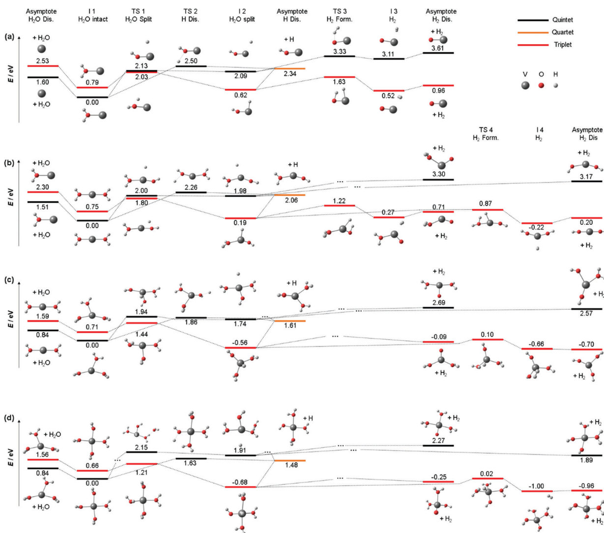
Fig. 3 Simplified potential energy surface of the lowest lying triplet state and quintet electronic state to follow the decomposition channels of (a) V + (H 2 O) (b) V + (H 2 O) 2 , (c) V + (H 2 O) 3 and (d) V + (H 2 O) 4 towards H 2 O loss, H 2 formation and H loss on the B3LYP/aug-cc-pVDZ level of theory. Only key steps of the PES for the decomposition are shown while missing minima or transition states are indicated via "...". H 2 O and H 2 loss PES of V + (H 2 O) similar to (a) have been reported previously. 47
