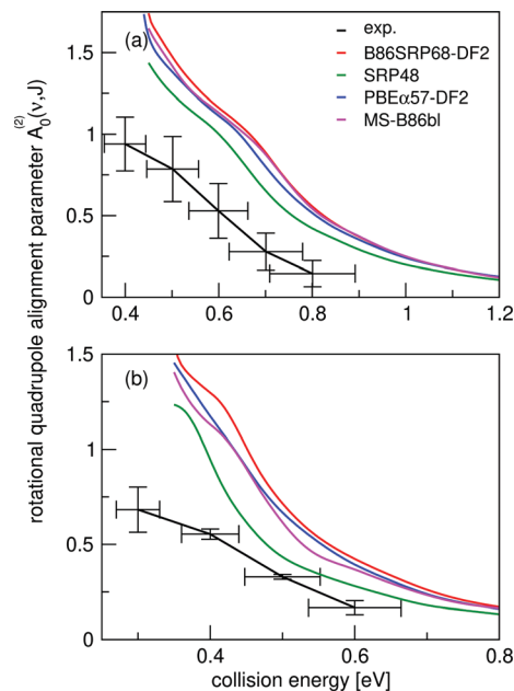
Fig. 14 Panel (a) shows rotational quadrupole alignment parameter, A_0^{(2)}(\nu=0, J=11) , and panel (b) shows the rotational quadrupole alignment parameter A_0^{(2)}(\nu=1, J=6) for D_2 reacting with Cu(111). Experimental results are shown in black. 49 Theoretical results using the QCT method are shown for the B86SRP68-DF2 (red), SRP48 10 (green), PBE \alpha 57-DF2 11 (blue), and the MS-B86bl 12 (magenta) DFs.
