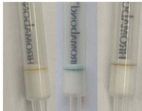
Fig. 7 Immobilizations of PV and \text{Cu}_2^{\text{II}} -PV on the top of C18ec cartridges at pH 6.50 ([HEPES] = 10 \text{ mM} ). Left: PV ( 2 \text{ mL} , 5 \mu\text{M} ; 10 \text{ nmol} ; dark yellow), middle: \text{Cu}_2^{\text{II}} -PV ( 2 \text{ mL} , 5 \mu\text{M} ; 10 \text{ nmol} ; detection zone: blue), right: \text{Cu}_2^{\text{II}} -PV + GlyP ( 2 \text{ mL} , 5 \mu\text{M} , 10 \text{ nmol} ; detection zone: dark yellow).
