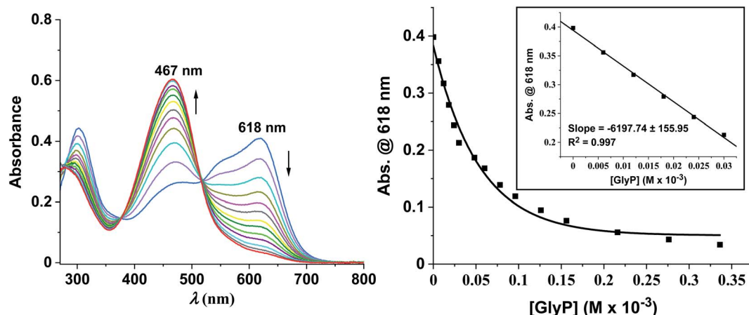
Fig. 5 Left: UV-vis spectra of titration of \text{Zn}^{\text{II}} -zincon ( 30 \mu\text{M} ; \lambda_{\text{max}} = 618 \text{ nm} ) with GlyP leading to metal-free zincon ( \lambda_{\text{max}} = 467 \text{ nm} ) at pH 7.20, [HEPES buffer] = 10 \text{ mM} . Right: Corresponding calibration curve ( [\text{Zn}^{\text{II}}\text{-zincon}] = 30 \mu\text{M} , [\text{GlyP}] = 0\text{--}30 \mu\text{M} ; LOD = 4.80 \mu\text{M} ( 811 \mu\text{g L}^{-1} ), R^2 = 0.997 ).
