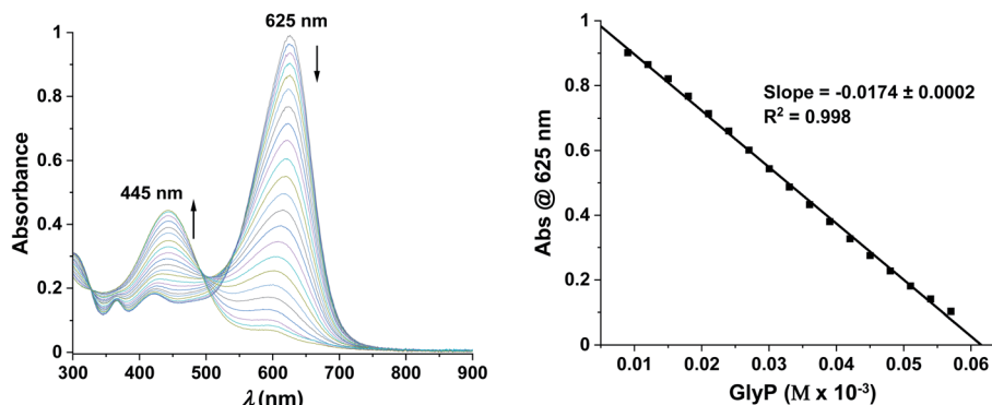
Fig. 6 Left: Changes of absorbance of \text{Cu}_2^{\text{II}} -PV ( 30 \mu\text{M} , \lambda_{\text{max}} = 625 \text{ nm} ) in the presence of GlyP ( 0\text{--}60 \mu\text{M} ) at pH 6.50, [HEPES buffer] = 10 \text{ mM} ; \lambda_{\text{max}} (PV) = 445 \text{ nm} . Right: Calibration curve with an LOD of 2.50 \mu\text{M} ( 422 \mu\text{g L}^{-1} ) ( R^2 = 0.998 ).
