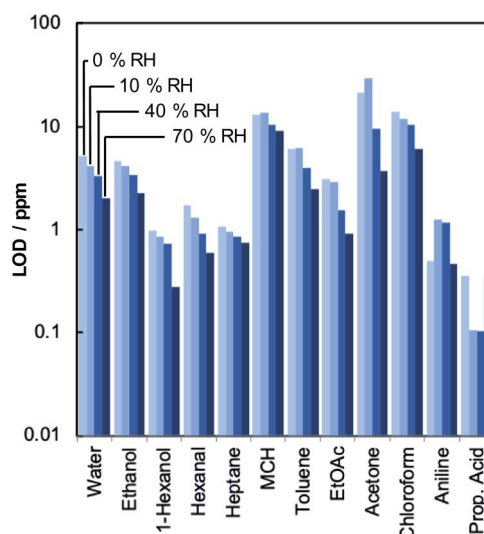
Fig. 3 Limit of detection (LOD) of a 2100 droplet nanoparticle ZIF-8-MSS sensor fabricated by inkjet deposition towards various analytes determined at 25^\circ\text{C} and humidity levels from 0% RH (light blue) to 70% RH (dark blue). MCH = methylcyclohexane; EtOAc = ethyl acetate; prop.acid = propionic acid.
