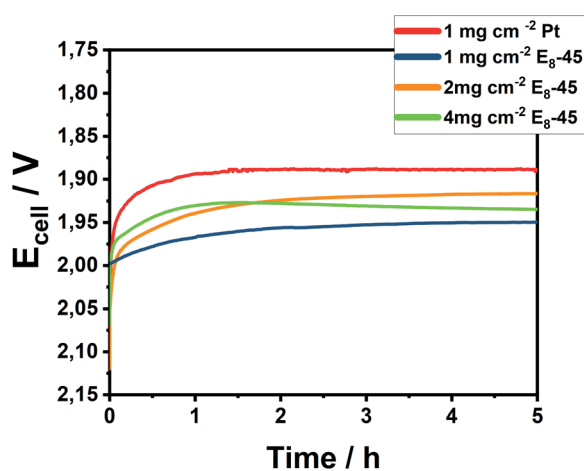
Fig. 6 Chronopotentiometry of Pt/C and \text{E}_8\text{-45/C} at a catalytic loading of 1–4 \text{mg cm}^{-2} at 80 ^{\circ}\text{C} for 5 h at an applied current of 1 \text{A cm}^{-2} .
